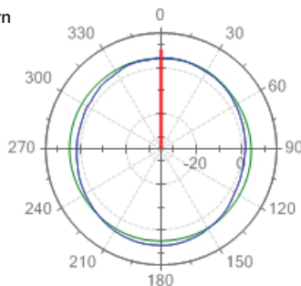
E-Plane Pattern
