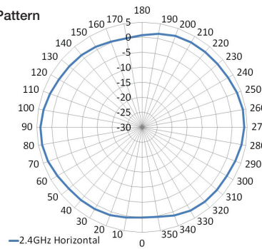
E-Plane Pattern
