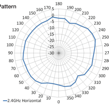
E-Plane Pattern
